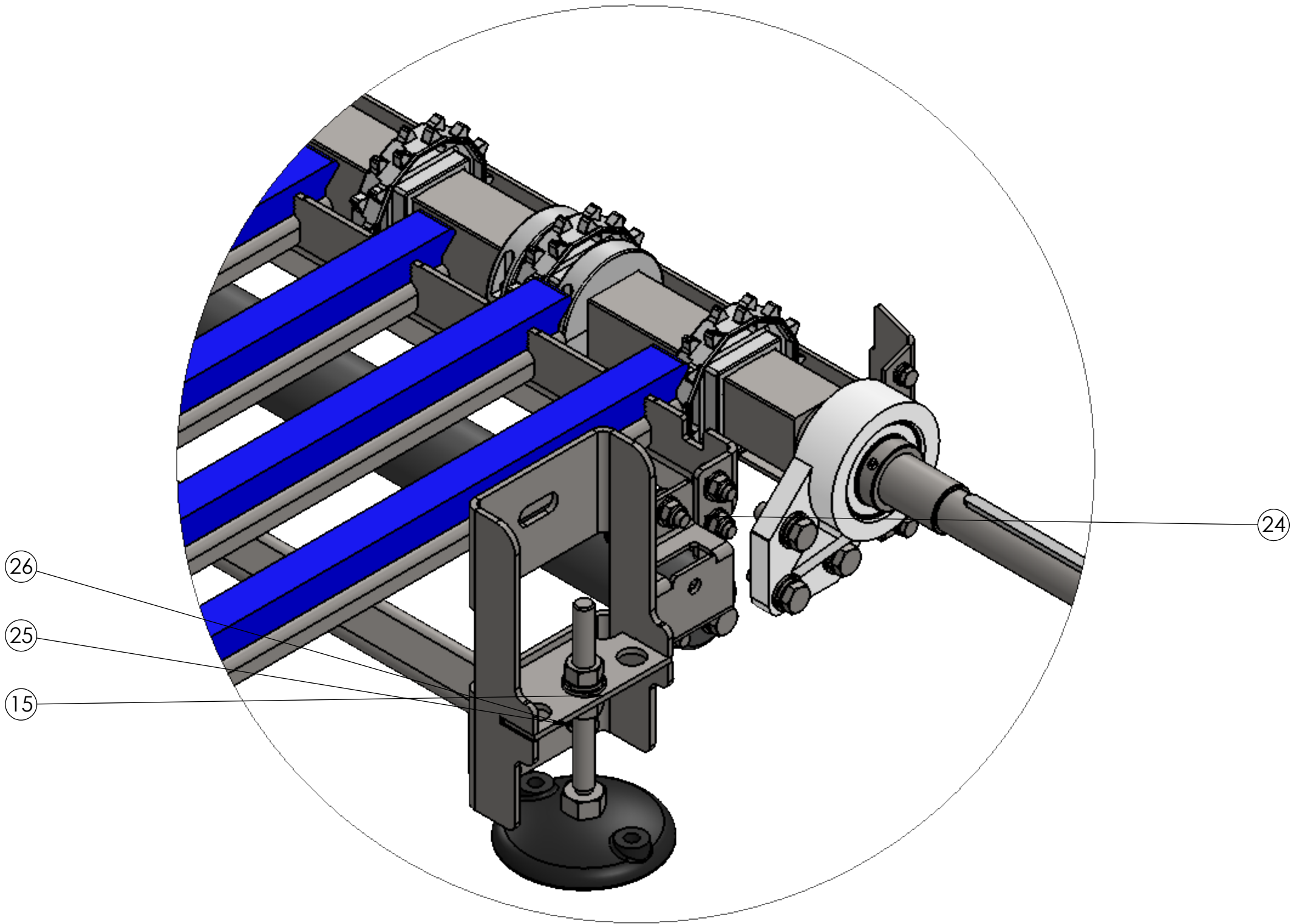
ISOMETRIC KEY / 1:40 GUIDE ATTACHMENT
