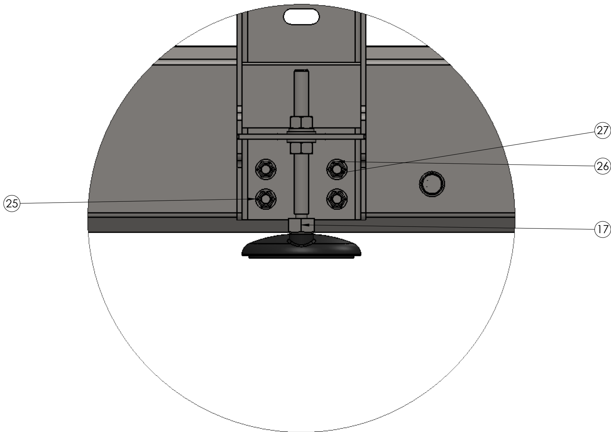
SIDE KEY / 1:25 SUPPORT ATTACHMENT
