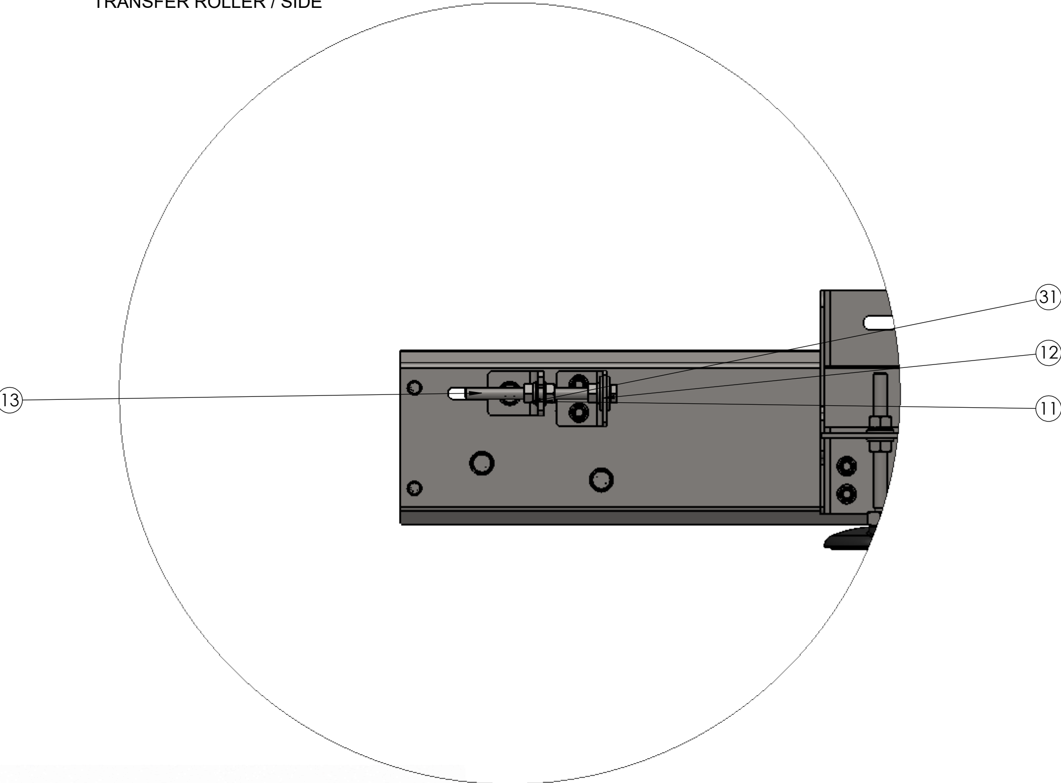
DETAIL C SCALE 0.3 : 1
