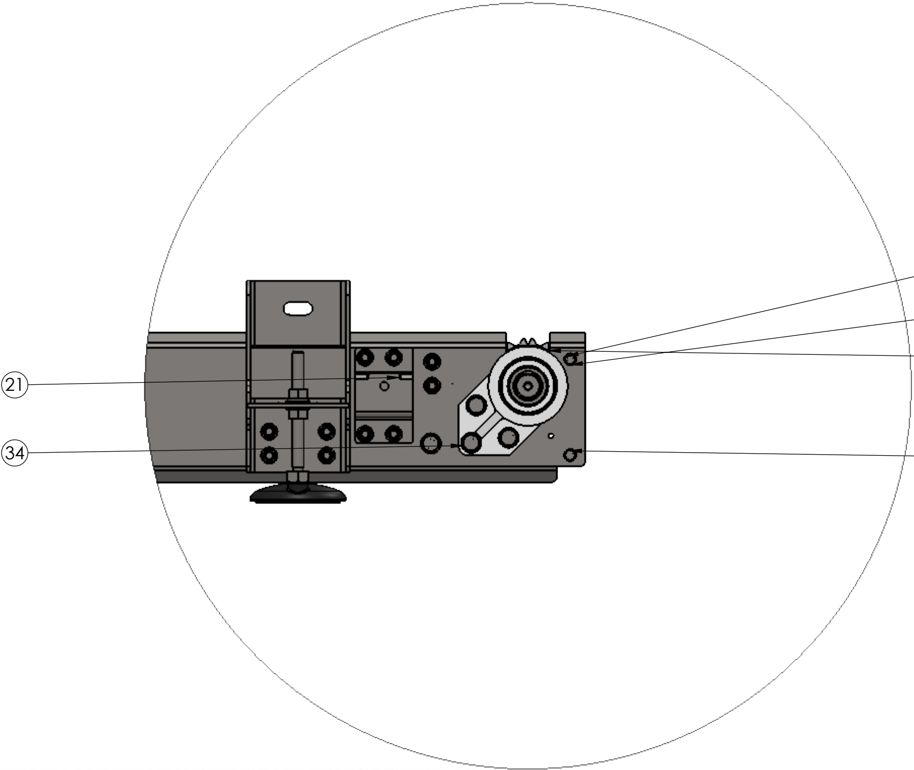
SIDE KEY / 1:25 DRIVE END / SIDE
