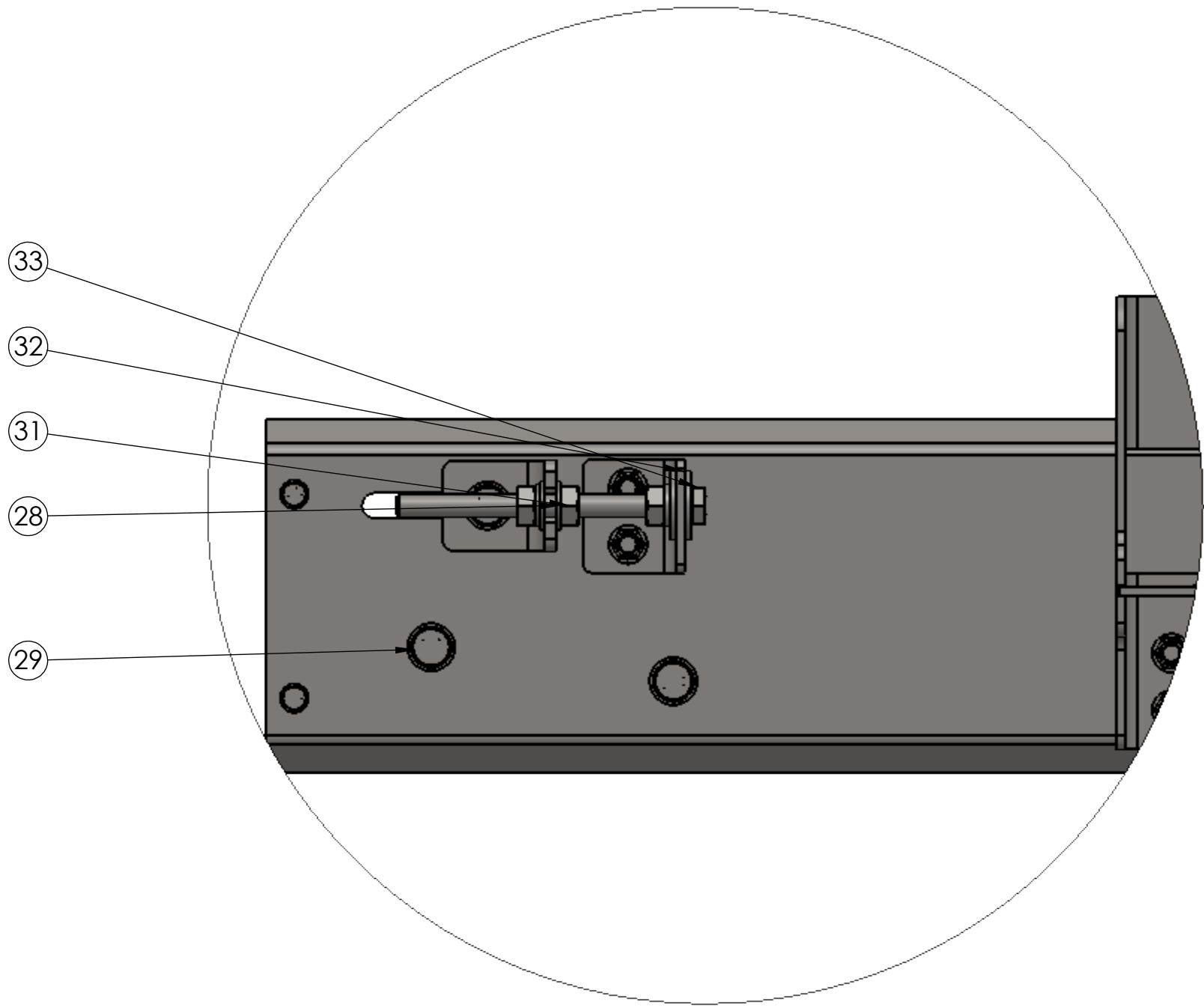
SIDE KEY / 1:25 LONG BOLT INTERFACE
