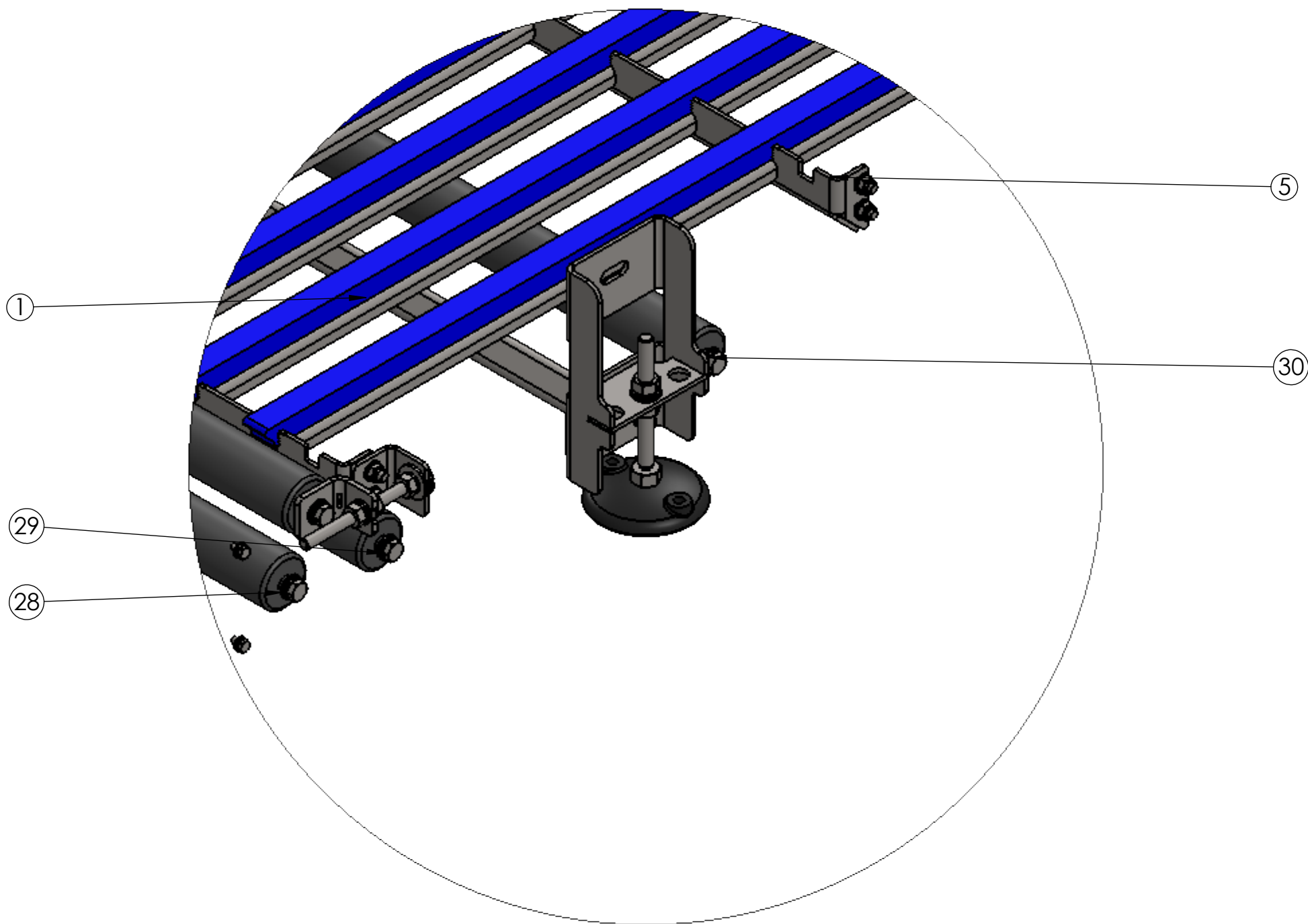
ISOMETRIC KEY / 1:40 SUPPORT / FRAME CONNECTION
